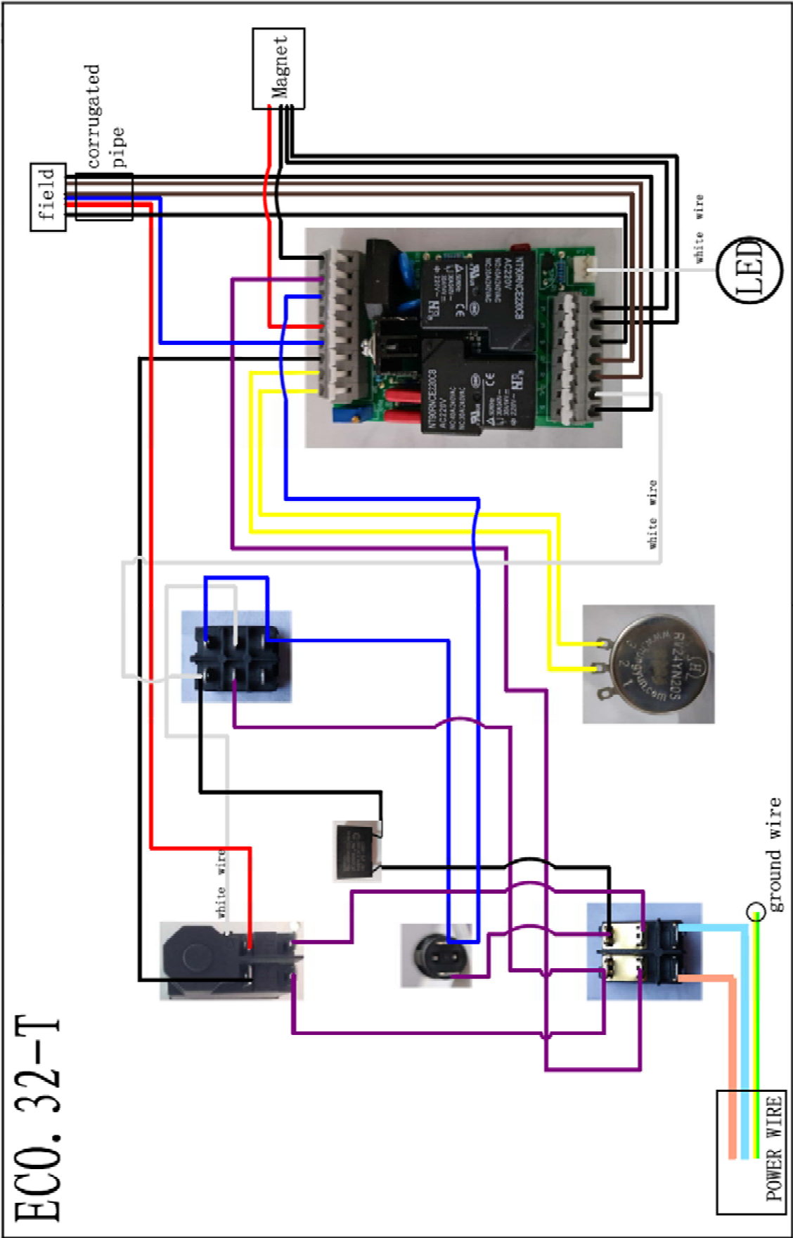
Wiring diagram
